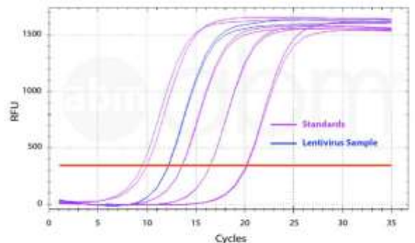
abm's qPCR Lentivirus Titer Kit enables easy visualization of viral titers. A lentivirus sample (blue) was processed following the protocol for the qPCR Lentivirus Titer Kit (Cat. No. LV900) and amplified in a qPCR reaction along with standards included in the kit (purple).
